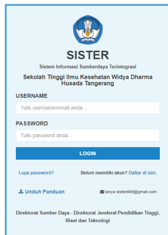
Gambar 1. Tampilan SISTER
